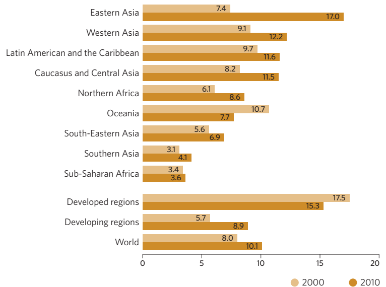
Domestic material consumption per capita, 2000 and 2010 (tons per capita)
